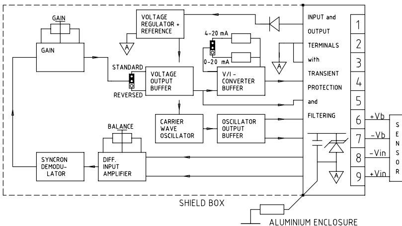
PCB Block diagram and Connection setups
