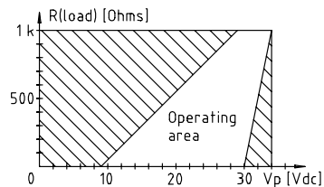
2-wire 4-20 mA load related to supply voltage
